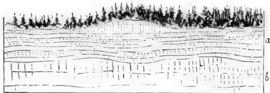
FIG. 9. SECTION IN CLIFFS NORTH OF CAPE BALL. a. Stratified sandy deposits. b. Imperfectly stratified clays.
