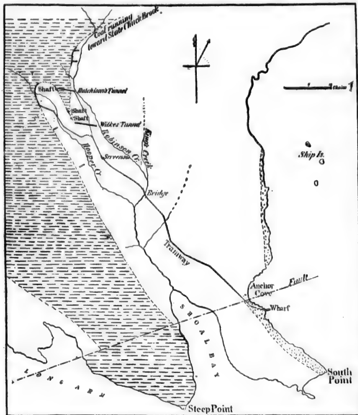
FIG. 4. PLAN OF COWITZ COAL MINE AND VICINITY, SKIDEGATE, Showing the Openings Made on the Coal and the Probable Course of the Seam. (The area shaded in broken lines is that occupied by Subdivision D. The area without shading is that of C., overlain by B., represented by dotted shading.) The Plan based chiefly on measurements made by Mr. Richardson in 1872.
