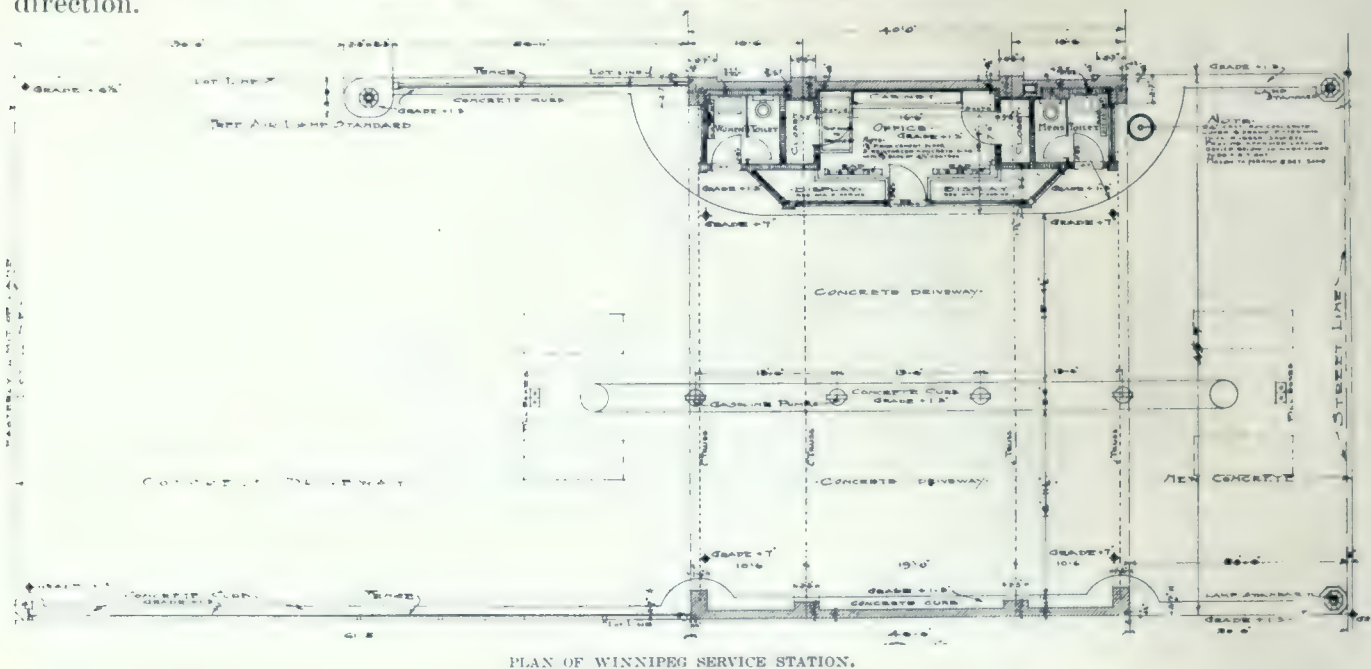
PLAN OF WINNIPEG SERVICE STATION.
