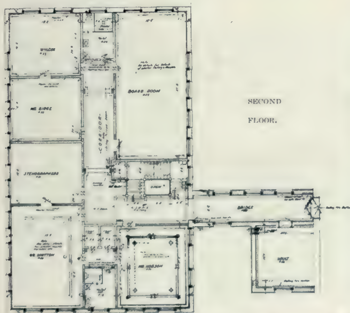
STEEL COMPANY OF CANADA'S OFFICE BUILDING, HAMILTON, ONT.
