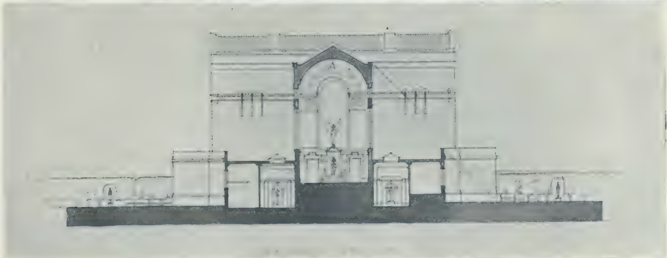
COMPETITIVE DESIGN, WAR MEMORIAL MUSEUM, REGINA, SASK.
