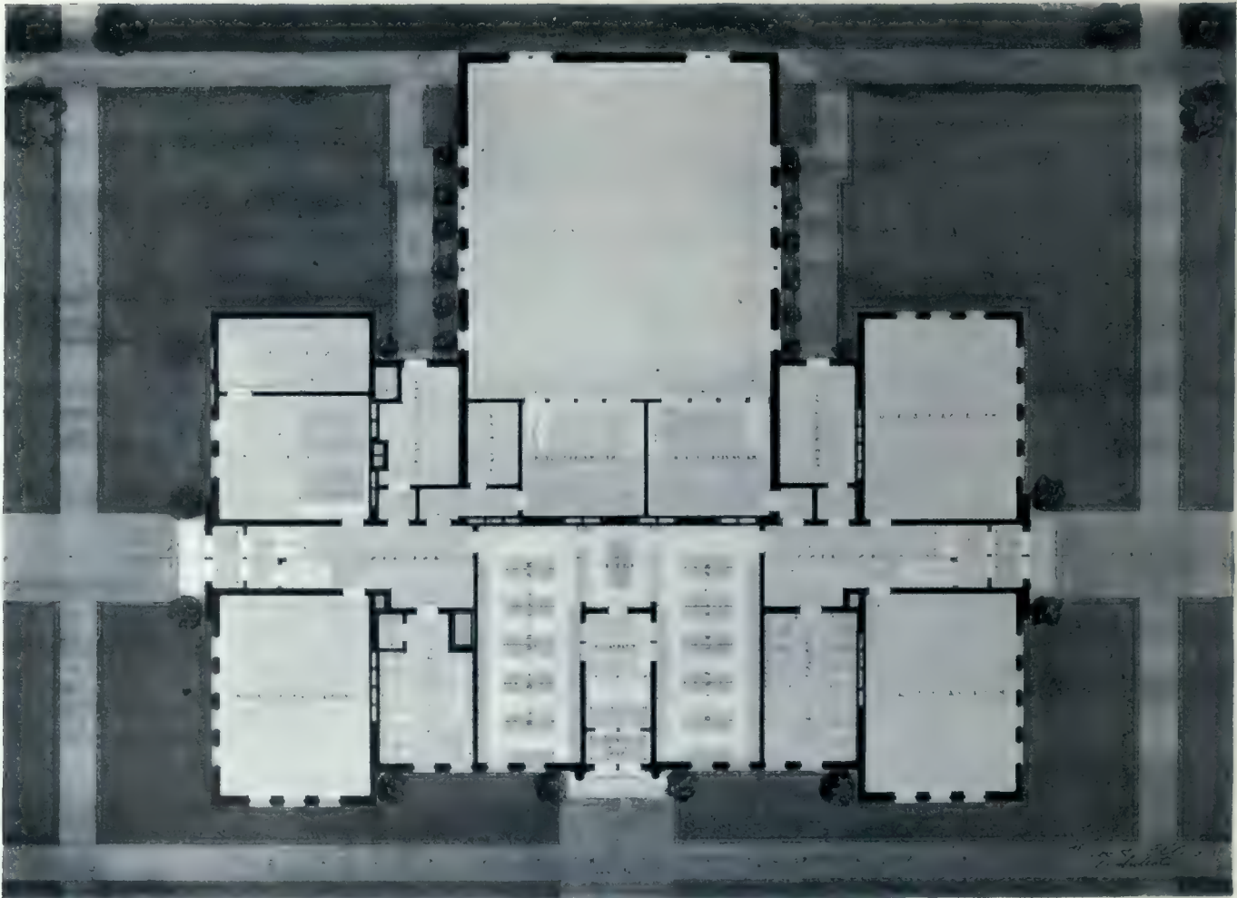
BASEMENT PLAN. COLLEGIATE INSTITUTE, BARRIE, ONT. ELLIS & ELLIS, ARCHITECTS.
