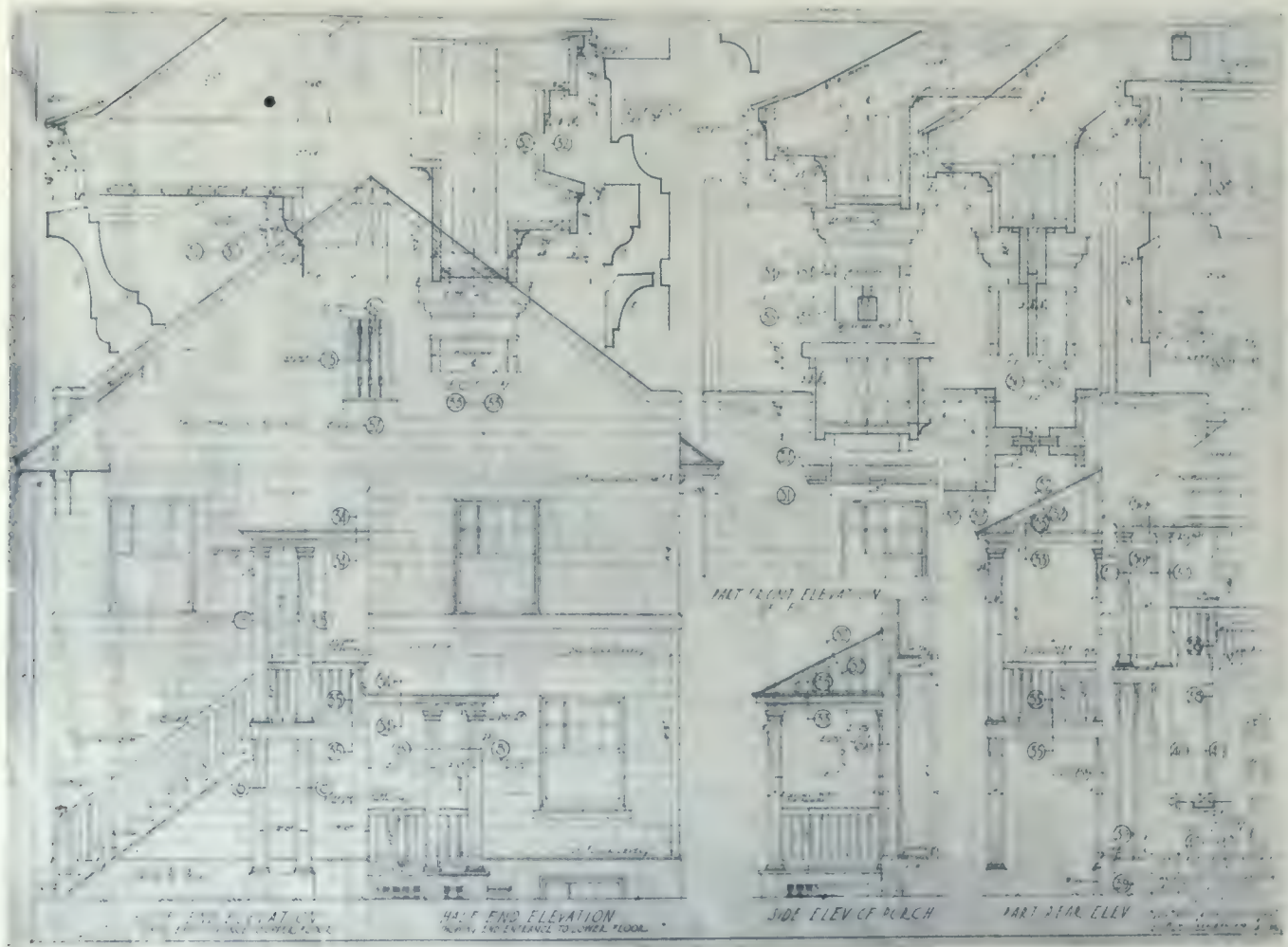
DETAILS OF TYPES F.2.1, F.2.2, DETACHED DWELLINGS, RE-HOUSING DEVELOPMENT, HALIFAX, N. S.
