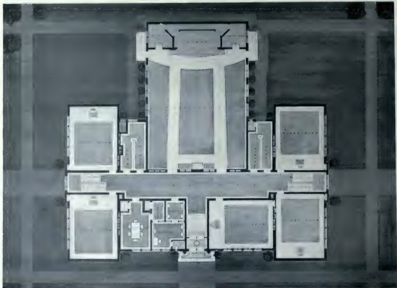
LOWER PLAN: GROUND FLOOR.
