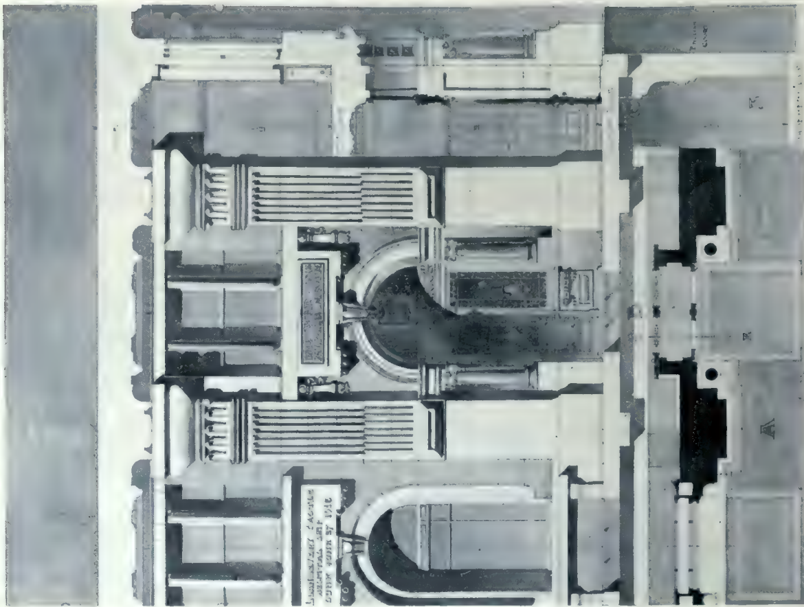
DETAIL.
