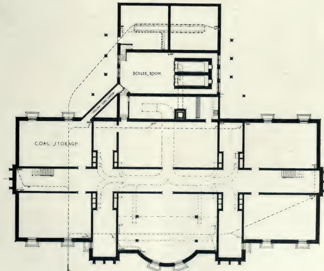
BASEMENT PLAN.
