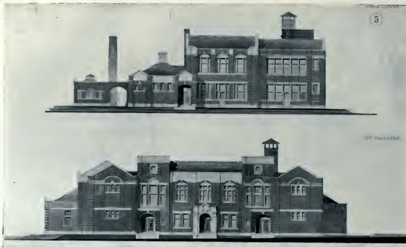
FRONT AND SIDE ELEVATIONS.
