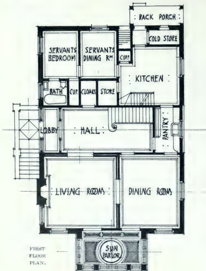
RESIDENCE OF A. J. WOOD, ESQ., WESTMOUNT, QUEBEC. SEPTIMUS WARWICK, F.R.I.B.A., ARCHITECT.
