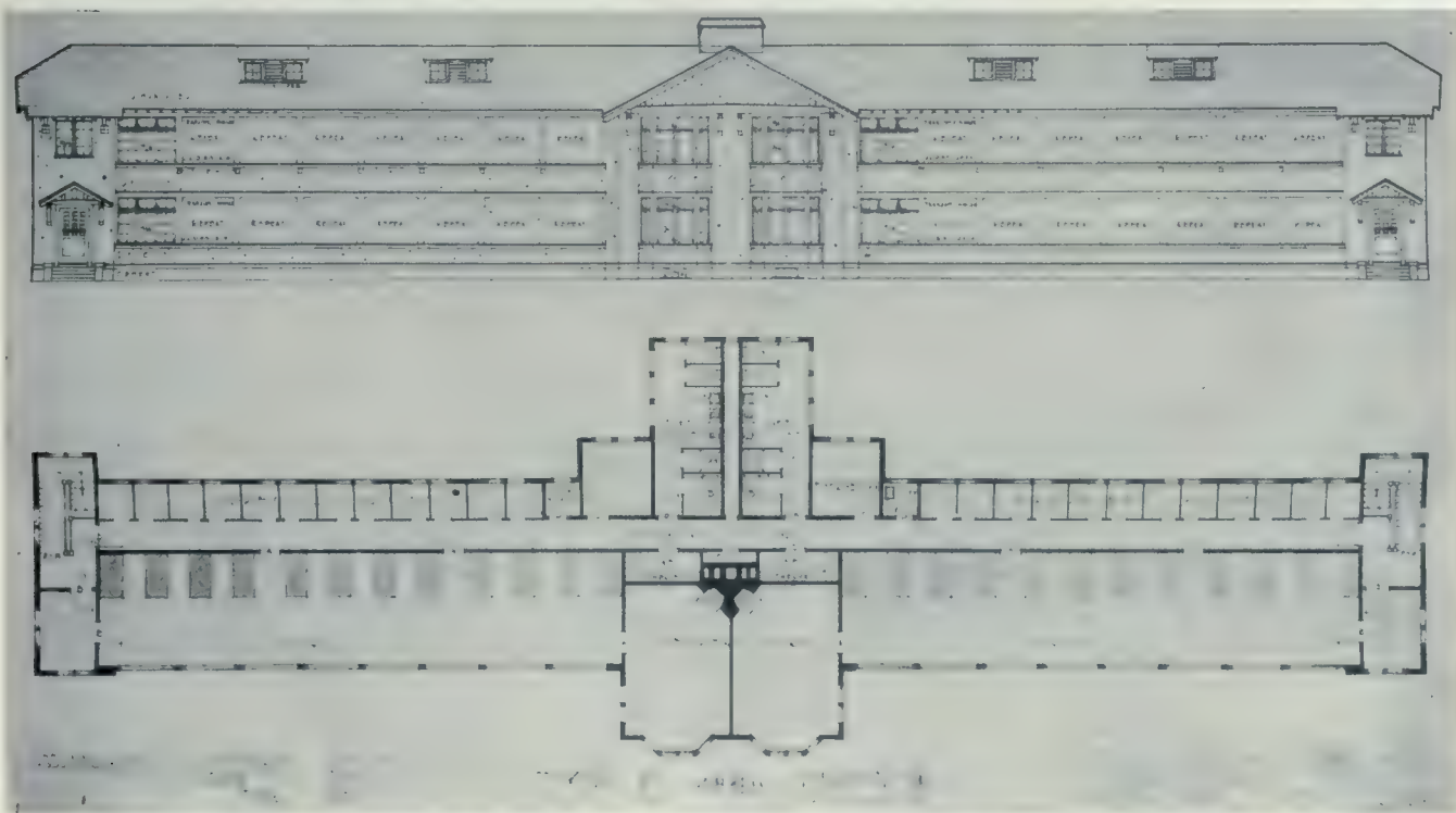
48 BED PAVILION, BYRON, ONT. ERECTED FROM STANDARD PLAN OF THE DEPARTMENT OF CIVIL RE-ESTABLISHMENT, OTTAWA. Watt & Blackwell, Supervising Architects.
