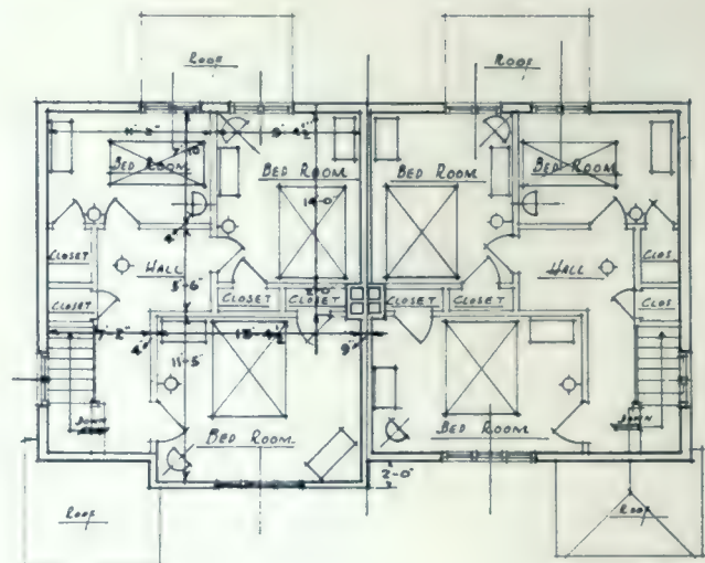
SUGGESTED SCHEME FOR FIVE ROOM SEMI-DETACHED HOUSE.
