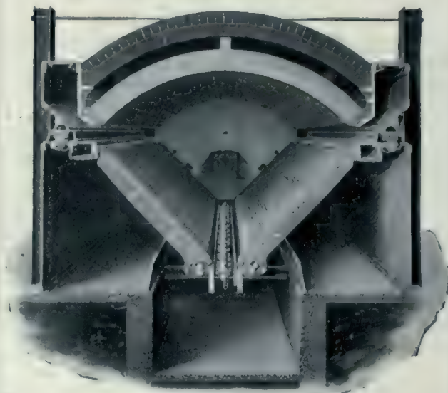
MURPHY AUTOMATIC FURNACE
