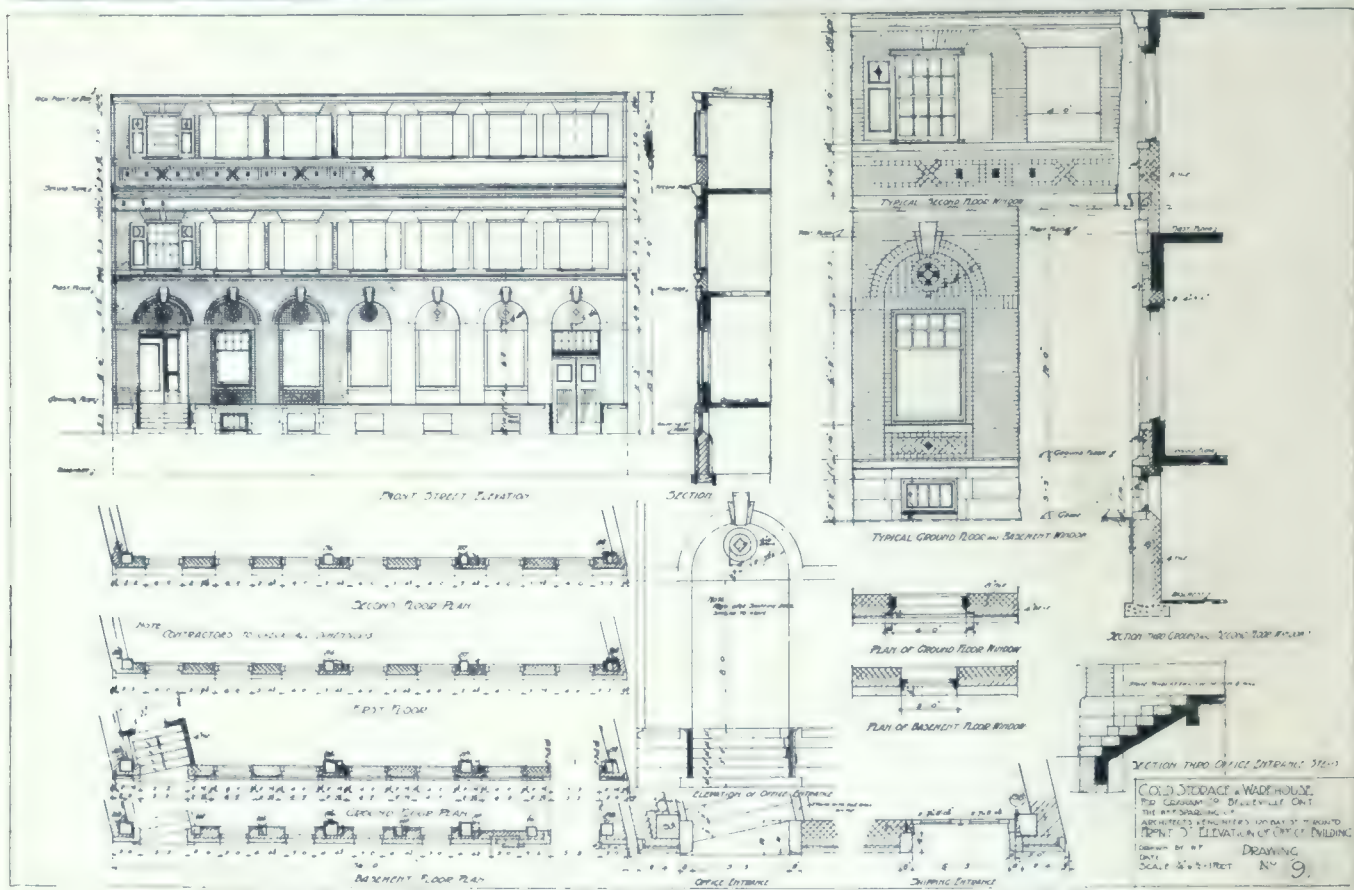
STREET ELEVATION, COLD STORAGE AND WAREHOUSE OF GRAHAM LIMITED, BELLEVILLE, ONT. W.M. F. SPARLING COMPANY, ARCHITECTS.
