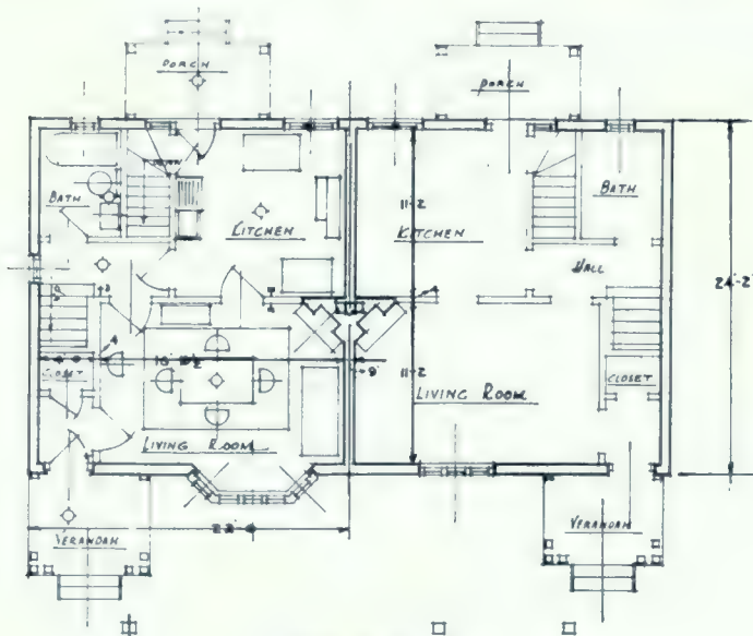
SUGGESTED SCHEME FOR FIVE ROOM SEMI-DETACHED HOUSE.
