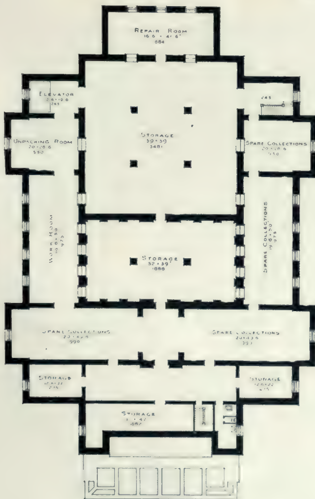
BASEMENT PLAN.
