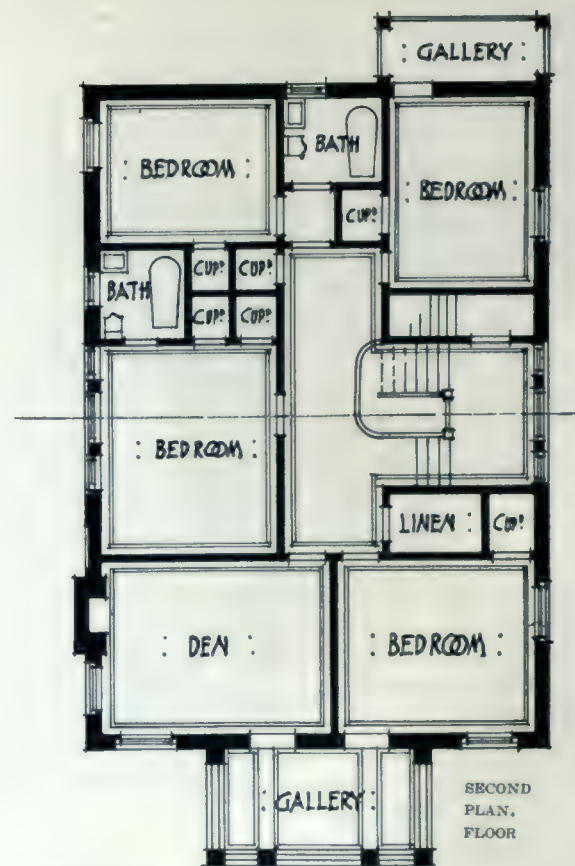
RESIDENCE OF A. J. WOOD, ESQ., WESTMOUNT, QUEBEC. SEPTIMUS WARWICK, F.R.I.B.A., ARCHITECT.
