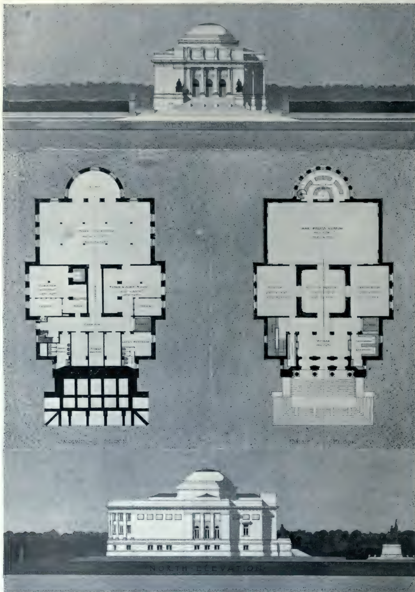
COMPETITIVE DESIGN, WAR MEMORIAL MUSEUM, REGINA, SASK.
