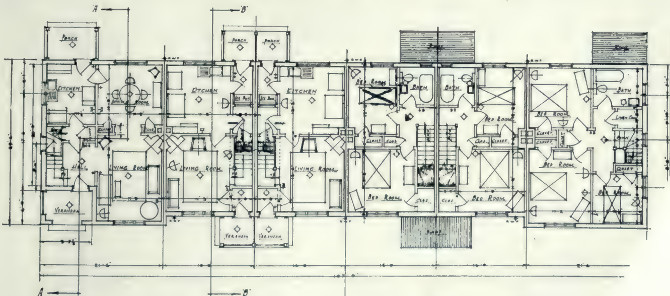
\frac{1}{8} INCH PLAN OF FIRST FLOOR.
