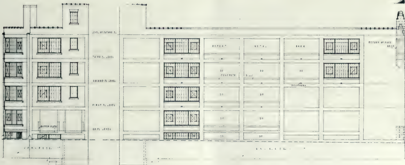
WEST ELEVATION.
