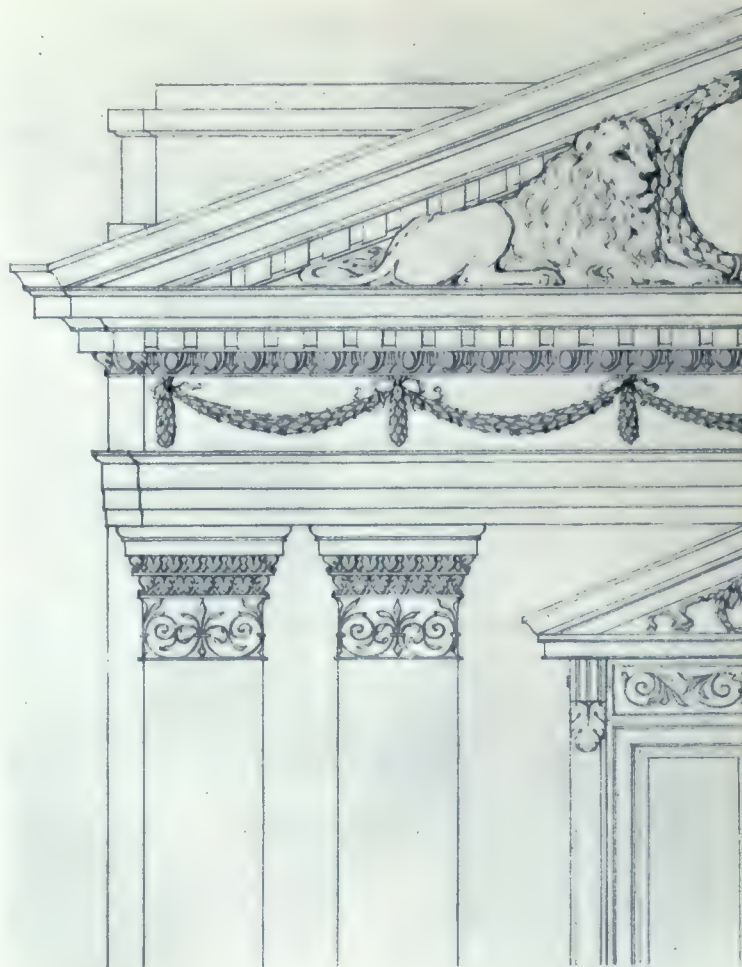
DETAIL.
