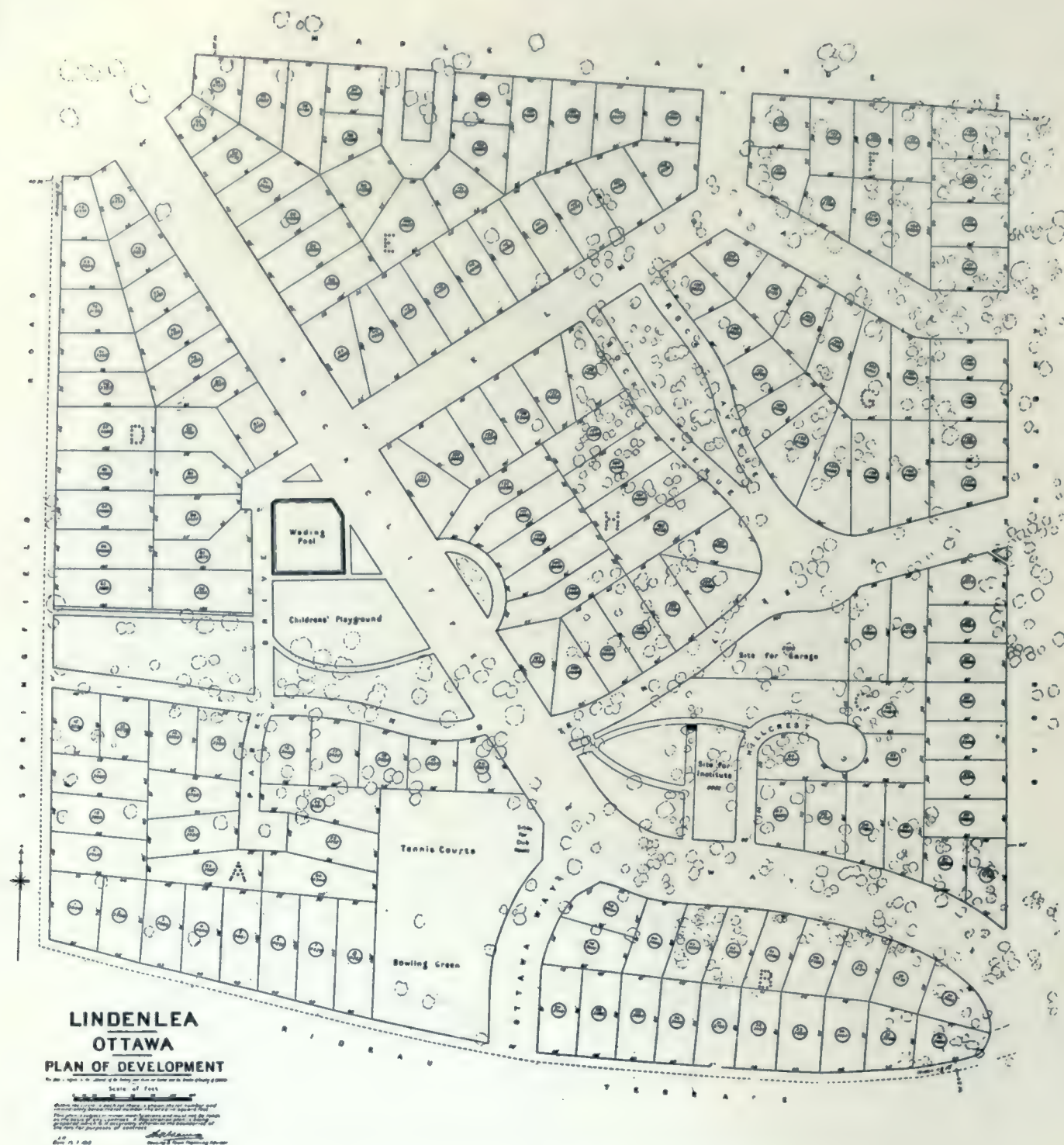
OTTAWA HOUSING COMMISSION'S PROPOSED DEVELOPMENT SCHEME.
