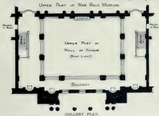
GALLERY PLAN. COMPETITIVE DESIGN, WAR MEMORIAL MUSEUM, REGINA, SASK.
