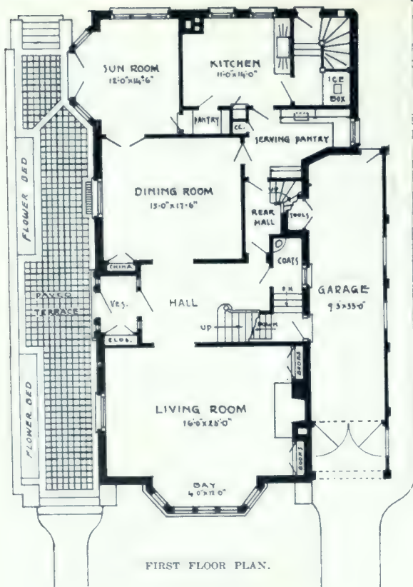
HOUSE ON DOUGLAS DRIVE, TORONTO.
