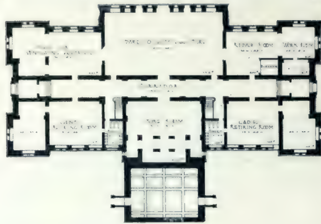
BASEMENT PLAN.
