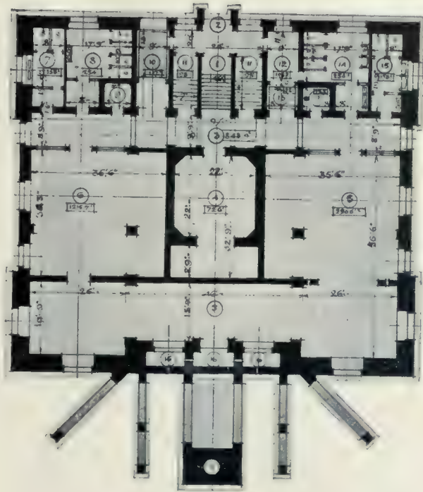
BASEMENT PLAN.
