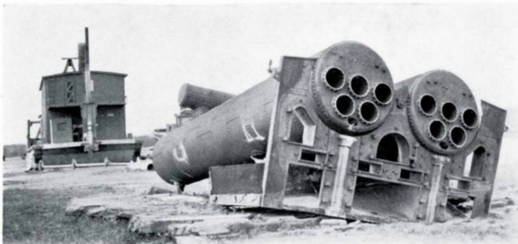
The Northcote's boilers at Cumberland House. Just in front of the dredge is the shaft of the stern wheel.
