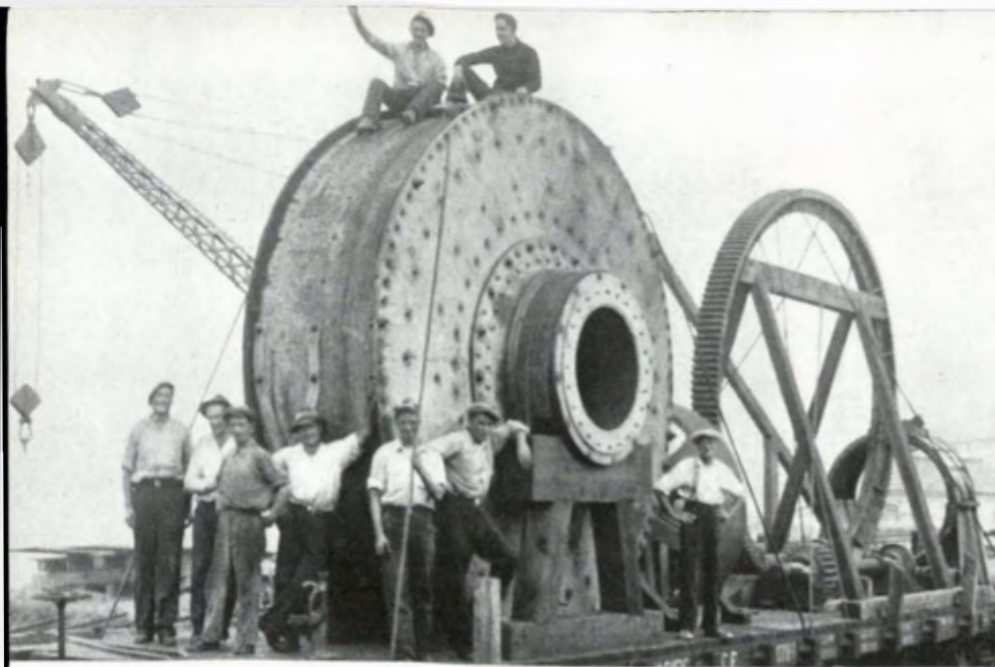
Part of a roller mill for Yellowknife.
